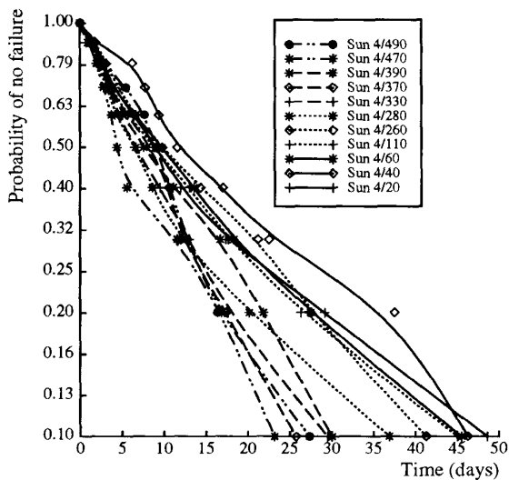
Figure 3: Semi-logarithmic Graph of Sun 4 Up-times.
