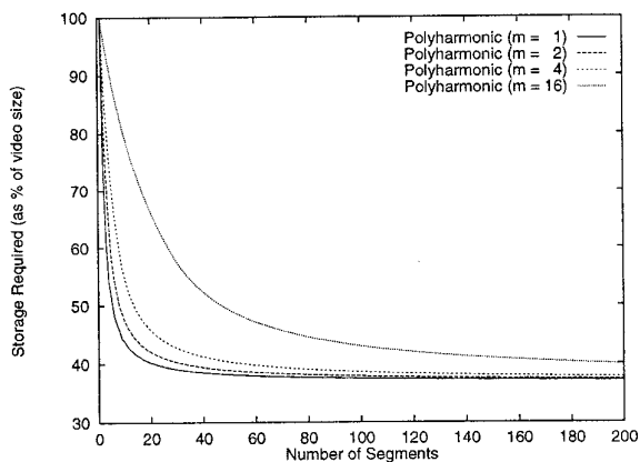
Figure 7: Storage requirements of polyharmonic broadcasting.
