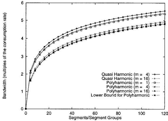
Figure 5: Bandwidth requirements of quasi-harmonic and polyharmonic broadcasting. The numbers on the x -axis represent number of segments for QHB and number of groups of m segments for PHB.
