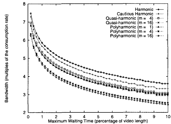
Figure 6: Bandwidth versus maximum waiting times for the quasi-harmonic and polyharmonic broadcasting protocols.
