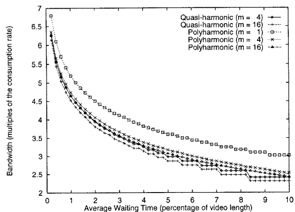
Figure 8: Bandwidth versus average waiting times for polyharmonic and quasi-harmonic broadcasting.
