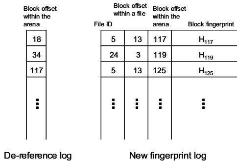
Figure 5. Data structures for logging recent clients' activities.
